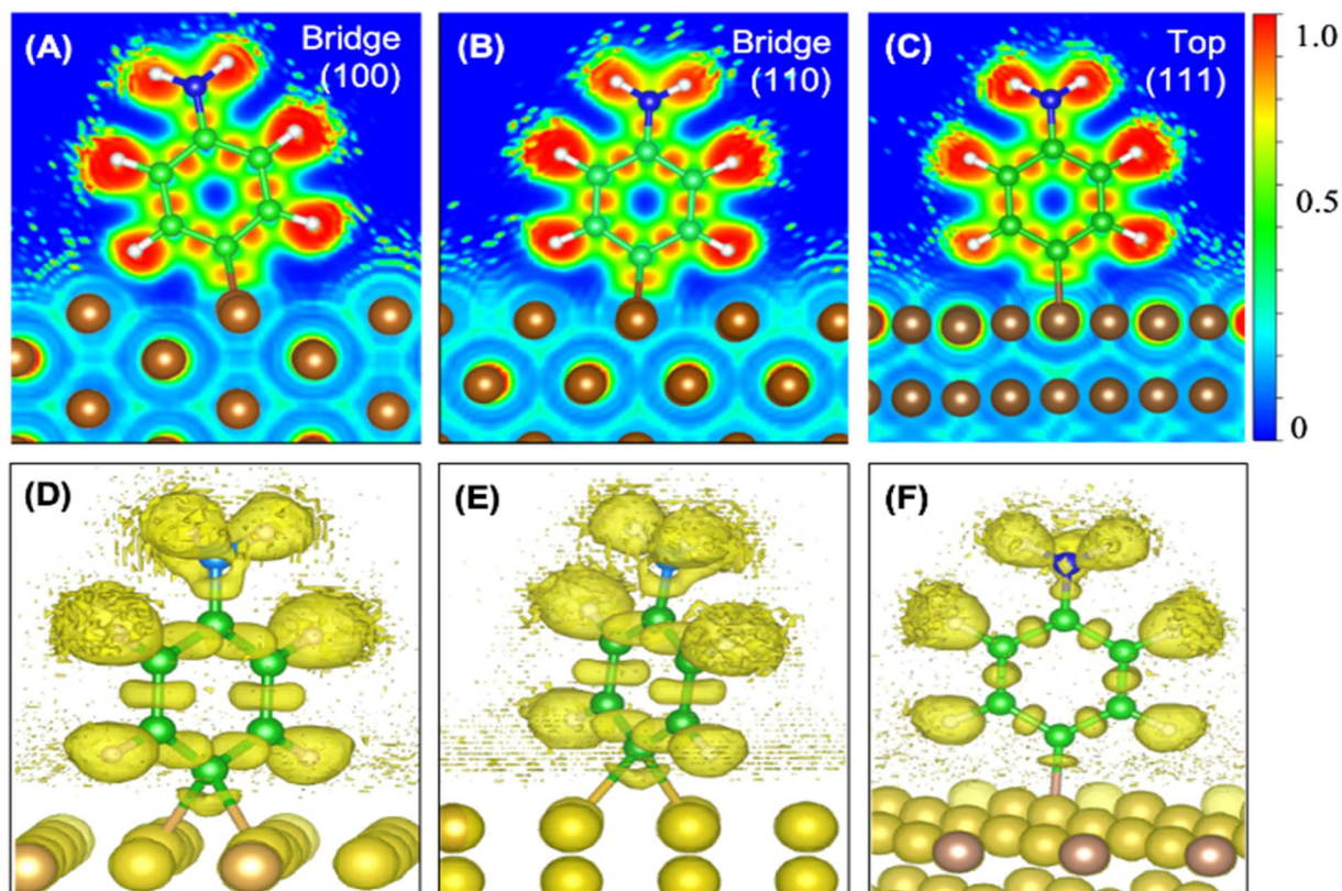
Fig. 3 2D ELF plots along the phase containing the Cu–C chemical bond on (A) Cu(100), (B) Cu(110), and (C) Cu(111). ELF isosurfaces ( \eta = 0.8 \text{ eÅ}^{-3} ) for an aminophenyl group on (D) Cu(100), (E) Cu(110), and (F) Cu(111). Nitrogen (blue), carbon (green), hydrogen (white), and copper (orange).
