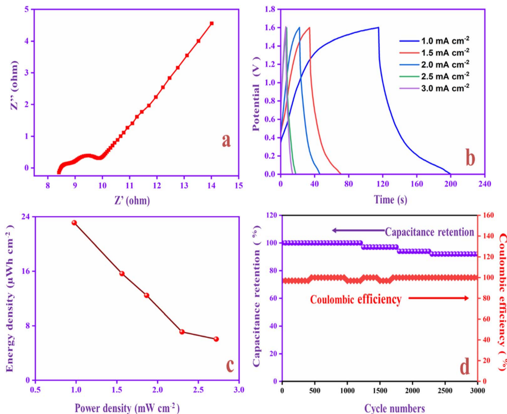
Fig. 14 (a) EIS study, (b) GCD, (c) Ragone plot and (d) cycling stability and coulombic efficiency of the AC/PVA- \text{H}_2\text{SO}_4 /PANI-CQD-Cu device (circular point: capacitance retention; diamond point: coulombic efficiency).
