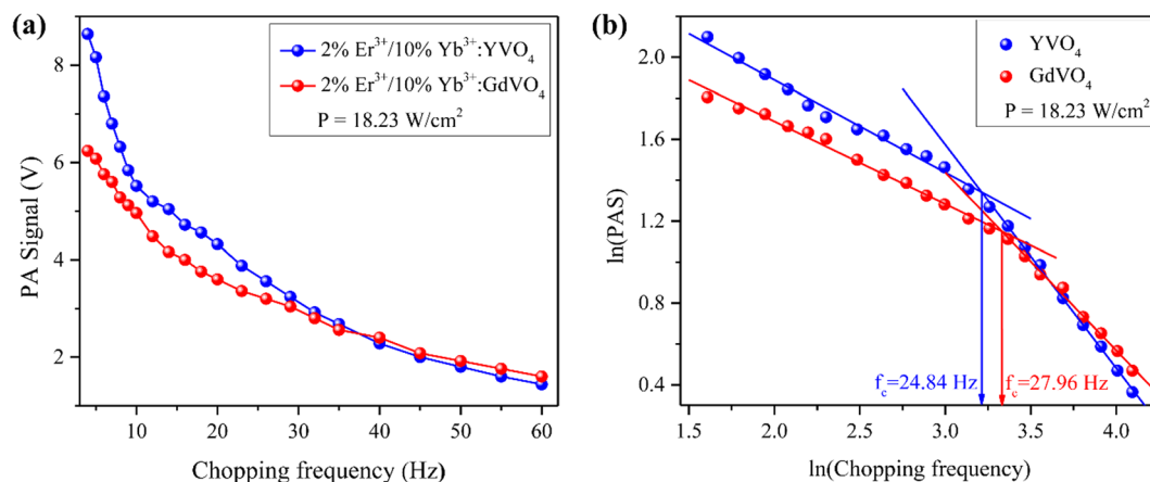
Fig. 9 (a) Variation of the photoacoustic signal amplitude with chopping frequency at an excitation power density of 18.23 \text{ W cm}^{-2} and (b) \ln(\text{chopping frequency}) – \ln(\text{PA signal}) graph for transition frequency calculation.
