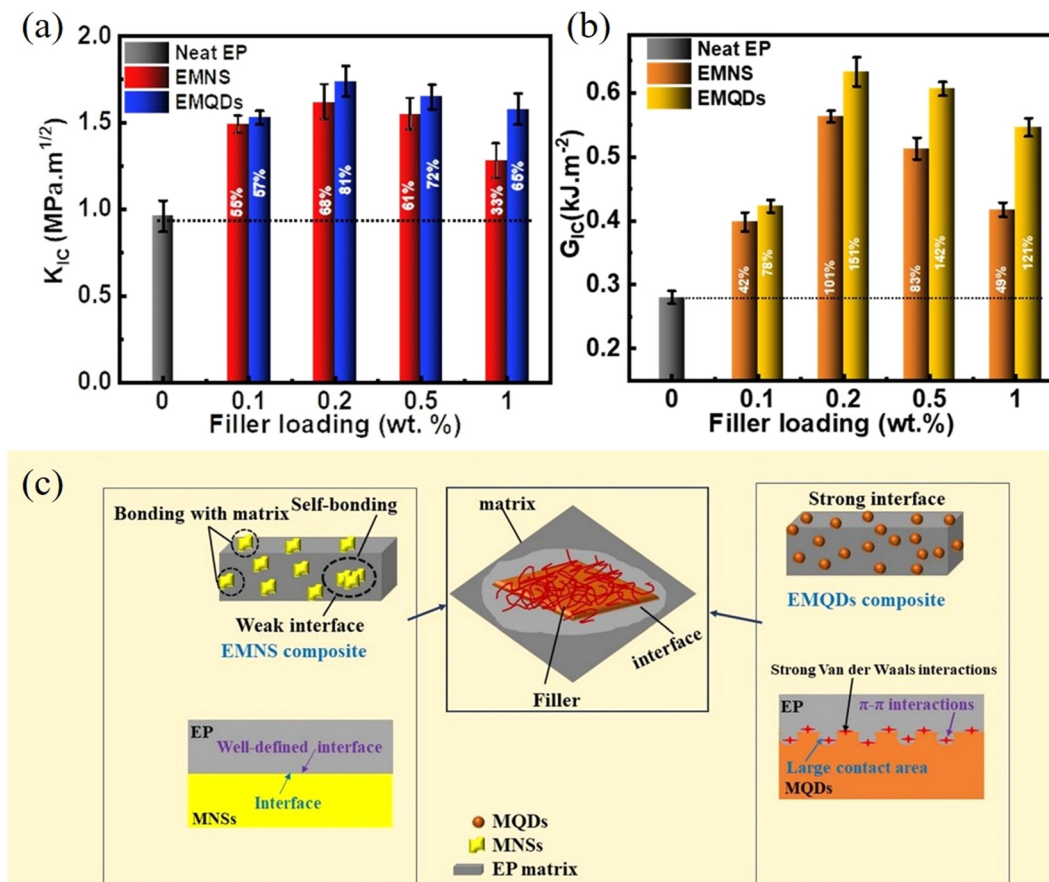
Fig. 26 (a) K_{1C} and (b) G_{1C} of neat epoxy, epoxy/MNSs (EMNS) and epoxy/MQDs (EMQDs) nanocomposites. (c) Interfacial interactions of EMNS and EMQDs. Reproduced with permission from ref. 241. Copyright 2021 Elsevier.
