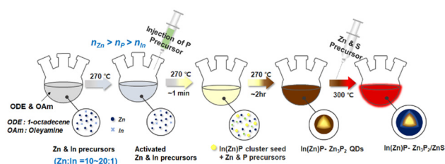
Fig. 1 Schematic of the \text{In}(\text{Zn})\text{P} seed-mediated synthesis process for \text{Zn}_3\text{P}_2 QDs using In precursor as a limiting agent and the subsequent overgrowth of the \text{ZnS} shell.
