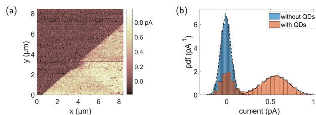
Fig. 3 Peak force tapping pcAFM measurements on QD monolayer on ITO/glass. (a) Current map for a bias of 500 mV and an irradiance of 50 W cm -2 (delivered through the 10\times objective) along an edge of the QD layer. (b) Histogram (bars) of the measured current values on the QDs (red) and on ITO (blue), scaled as probability density function (pdf). The black dotted lines show normal distributions with \mu = -0.01 pA and \sigma = 0.06 pA and \mu = 0.56 pA and \sigma = 0.16 pA.
