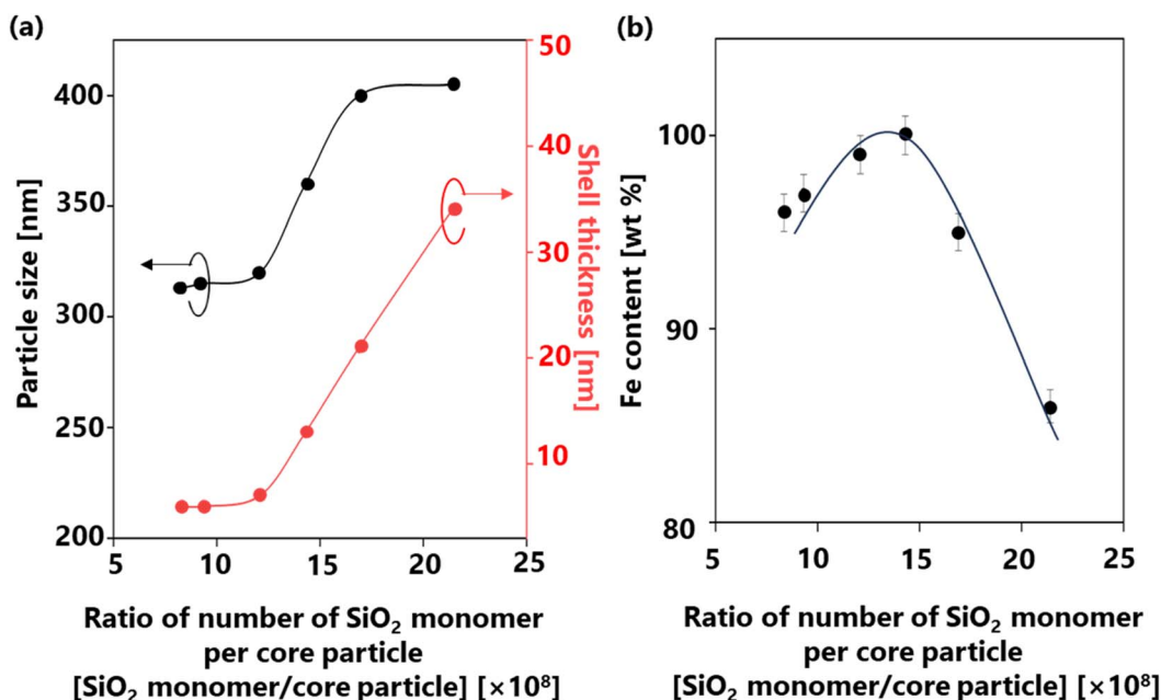
Fig. 7 Correlation between the number of SiO 2 monomer per core particle ratios on the (a) particle size and shell thickness and (b) α-Fe content in the Fe@SiO 2 particles.
