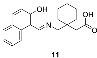
Fig. 13 Structure of Schiff base 11.
