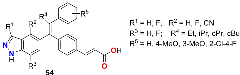
Fig. 37 Structure of fluorinated indazole derivatives 54.
