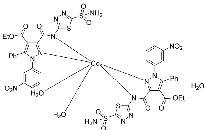
(Diaquabis(ethyl-1-(3-nitrophenyl)-5-phenyl-3-(5-sulfamoyl-1,3,4-thiadiazol-2-yl)carbamoyl)-1H-pyrazole-4-carboxylate)cobalt(II) monohydrate
