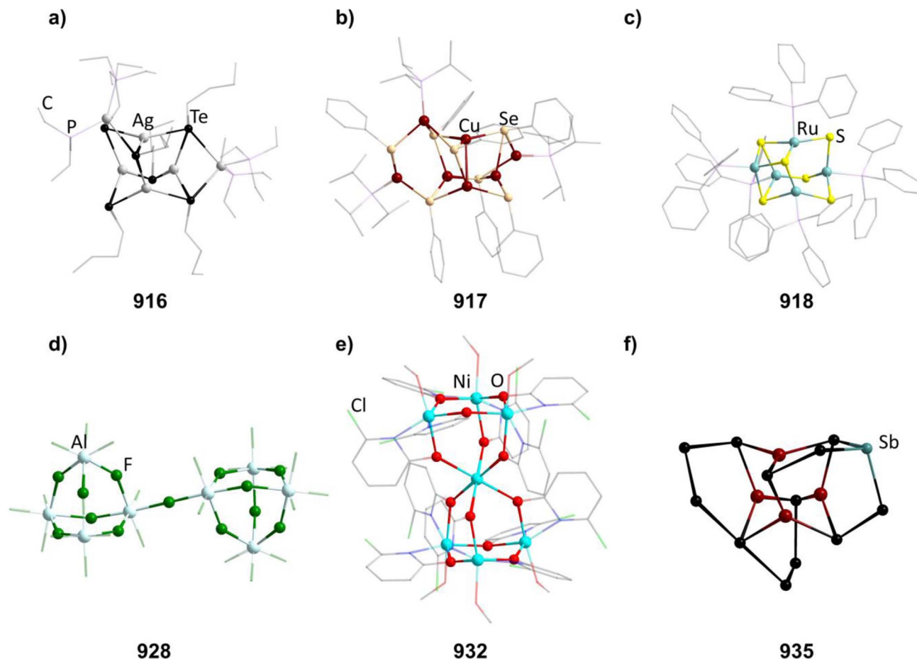
Fig. 20 Examples of compounds with an extended adamantane-type structure: [\text{Ag}_4\{\text{Ag}(\text{PET}_3)_2\}_2(\text{Te}^r\text{Bu})_6] ( 916 , top left (a)), [\text{Cu}_4(\text{CuP}^i\text{Pr}_3)_3(-\text{SePh})_7] ( 917 , top center (b)), [\mu_3-(\text{RuPPh}_3)(\text{RuPPh}_3)_4\text{S}_6] ( 918 , top right (c)), [\text{H}_3\text{tren}]_4[\text{Al}_4\text{F}_{17}]_2\text{F]OH} ( 928 , bottom left (d)), [\text{Ni}\{\text{Ni}(\text{chp})_2\text{MeOH}\}_6]\text{Cl}_2 ( 932 , bottom center (e)) and [\text{Et}_4\text{N}]_3[\text{Cu}_4\text{Sb}(\text{Te}_7)(\text{Te}_2)_2\text{Te}] ( 935 , bottom right (f)). Hydrogen atoms and counterions, if present, are omitted for clarity.
