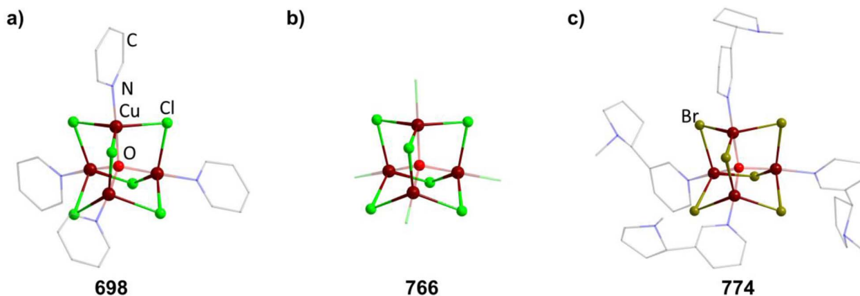
Fig. 16 Examples of adamantane-type clusters with a central μ 4 -oxygen atom, Cu in the Q position and group 17 atoms in the E position: [μ 4 -O{Cu(Py) 4 }] 4 Cl 6 (698, left (a)), [Me 4 N] 4 [μ 4 -O{CuCl 4 }] 4 Cl 6 (766, center (b)) and [μ 4 -O{Cu(nicotine)} 4 Br 6 ] (774, right (c)). Hydrogen atoms and counterions, if present, are omitted for clarity.
