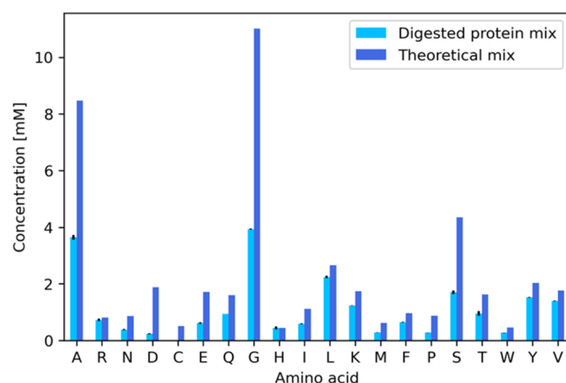
Fig. 5 Bar plot of the concentration of each AA in the digestion product of silk fibroin, \beta -lactoglobulin A and glucagon. Light blue represents the HPLC-MS/MS quantification result of the digestion product. Dark blue represents the theoretical concentration, for comparison.
