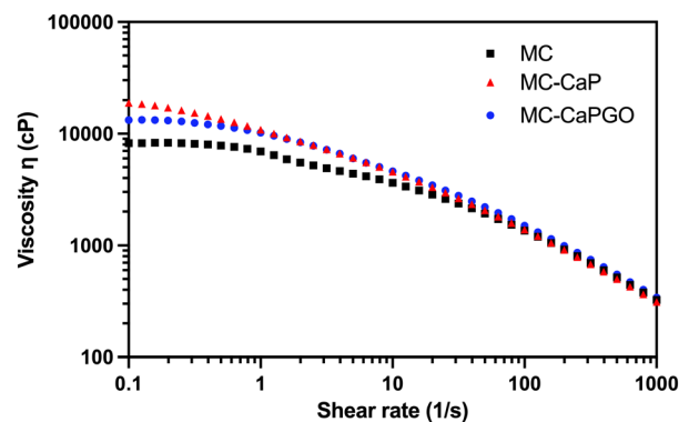
Fig. 2 Representative flow curves for MC, MC-CaP, and MC-CaPGO formulations. The tests were carried out at 20 °C, applying a shear rate ramp from 0.1 to 1000 s -1 .
