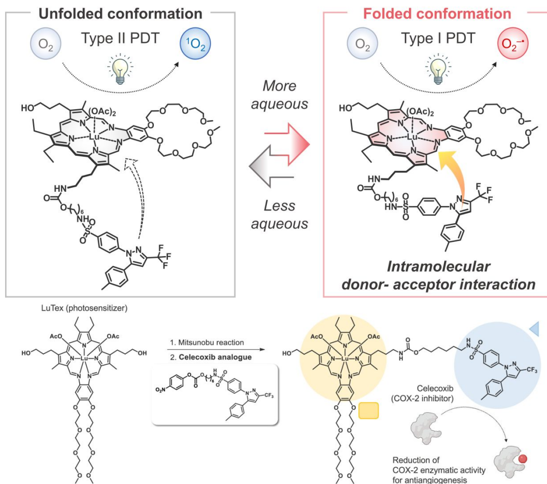
Figure 1 Schematic illustrates the interconversion between dominant type II and type I ROS generation, which is influenced by the surrounding medium as well as the chemical structures. Additionally, it presents a concise synthetic route to produce LuTex-derived conjugates of small molecule photosensitizers containing celecoxib (LuCXB).
