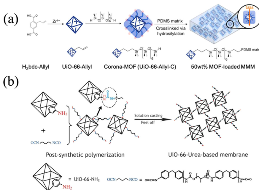
Figure 10 (a) Preparation of MMMs by crosslinking PDMS grafted-UiO-66-Allyl with the PDMS matrix. Adapted with permission from Yuji Katayama, Kyle C. Bentz, and Seth M. Cohen ACS Appl. Mater. Interfaces 2019 11 (13), 13029–13037. DOI: 10.1021/acami.9b02539. Copyright 2019 American Chemical Society. (b) Schematic illustration of MMMs prepared from grafting isocyanate-terminated polyurethane to UiO-66-NH 2 . Copyright 2016 John Wiley and Sons.
