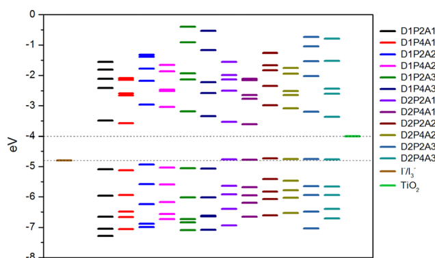
Fig. 1 Selected MOs energy levels for the designed dyes at the B3LYP/6-311+G(2d,p)/SMD level together with \text{TiO}_2 CB and \text{I}^-/\text{I}_3^- redox potential.
