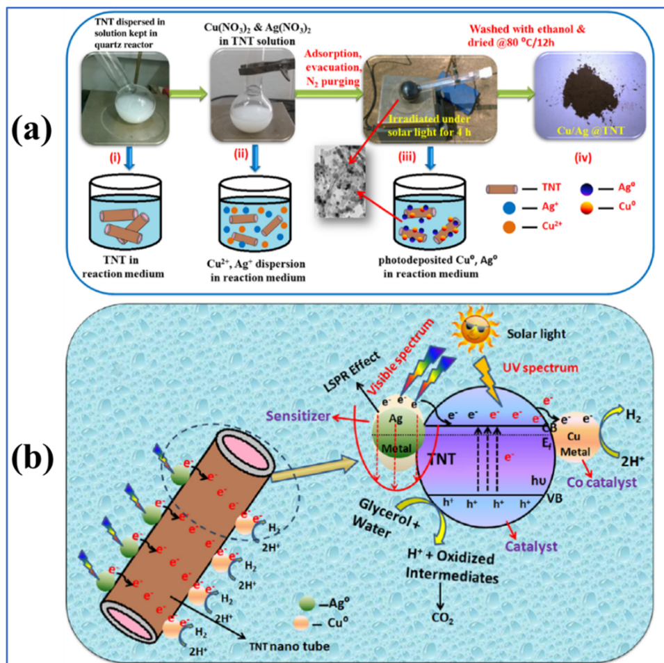
Fig. 6 (a) Schematic synthesis of Cu/Ag bimetallic deposition on titanium nanotubes (TNTs) and (b) charge separation and hydrogen evolution mechanism of as-synthesized Cu/Ag@ \text{TiO}_2 . Reproduced with permission from ref. 99. Copyright©2017, Elsevier Ltd.
