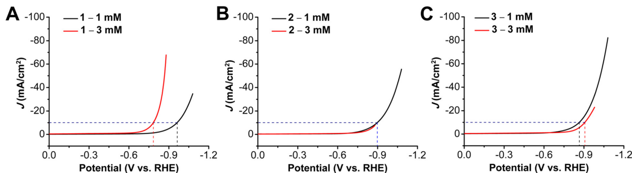
Fig. 3 LSVs for on HER performance of 1 mM and 3 mM ink solutions of complexes (A) 1 (B) 2 and (C) 3 . Obtained with 1\text{ cm}^2 carbon paper coated with a catalyst ink containing Vulcan carbon, Nafion, and given concentration of indicated complex as the working electrode. All experiments performed under \text{N}_2 saturation in 1.0\text{ M KOH} ; glassy carbon counter electrode, Hg/HgO reference electrode; 100\text{ mV s}^{-1} scan rate.
