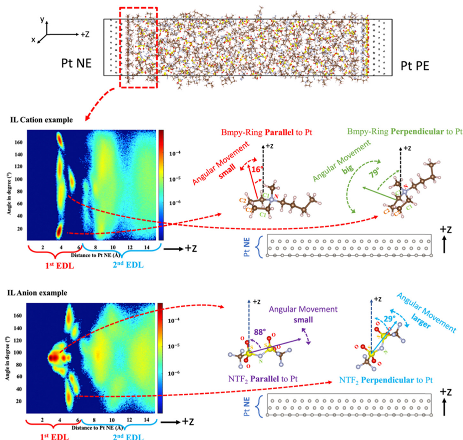
Fig. 5 Schematic of IL orientation distribution: using [Bmim] + and [NTf 2 ] - near the NE region (Pt Q = -8 e) as an example. For [Bmim] + , an angle close to 0° or 180° indicates that the cation ring tends to stay parallel to the electrode, and the angular movement of this molecule is usually small. If the angle of a cation is close to 90°, the molecule tends to remain perpendicular to the electrode, usually with big angular movement. For [NTf 2 ] - , an angle close to 90° suggests a parallel configuration with small angular movement, while an angle near 0° or 180° indicates a perpendicular configuration with larger angular movement.
