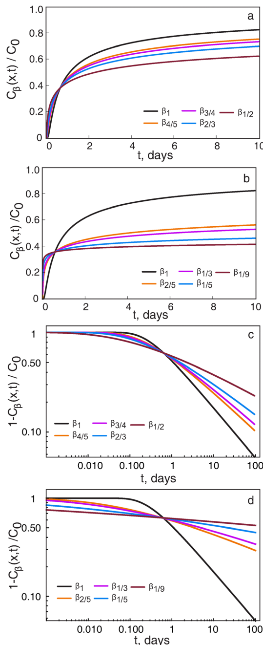
Fig. 2 Normalised BTCs (a and b) and residual BTCs (c and d) for both the Fickian and anomalous models. These solutions are based on diffusion through a 1 cm thick, porous material, i.e., x = 1 in our units. The linear plots illustrate that a decrease in the \beta value results in a sharper initial arrival of solute species compared to the Fickian case. The residual plots demonstrate that the long-time tails for the Fickian model decay strictly with a slope of -1/2 . Conversely, the long-time tails for \beta = 4/5, 3/4, 2/3, 1/2, 2/5, 1/3, 1/5 , and 1/9 decay with slopes of -2/5, -3/8, -1/3, -1/4, -1/5, -1/6, -1/10 and -1/18 , respectively.
