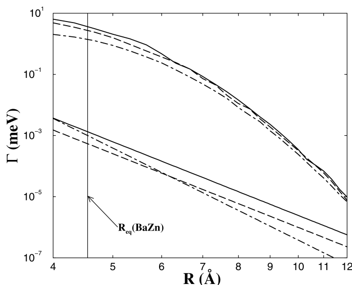
FIG. 1. Total ICD rates of BaZn resulting from Zn 3d sub-shell ionization as a function of the internuclear distance R . The vertical line indicates the equilibrium distance R_{eq} of the BaZn dimer. The three upper curves show the ab initio calculated results for \Gamma_0 , \Gamma_{\pm 1} , and \Gamma_{\pm 2} . The three lower curves show the quadrupole-dipole ( \Gamma_0 , \Gamma_{\pm 1} ) and the quadrupole-quadrupole ( \Gamma_{\pm 2} ) asymptotic approximations resulting from the Coulomb interaction (see text). Solid lines: 3d_0 vacancy; dashed lines: 3d_{\pm 1} vacancy; dash-dotted lines: 3d_{\pm 2} vacancy. The figure is taken from [47].
