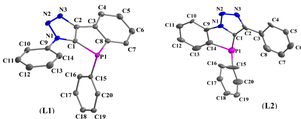
Fig. 1 Molecular structures of [C_6H_5\{1,2,3-N_3CC_6H_4C(PPh)\}] (L1) and [C_6H_4\{1,2,3-N_3C(Ph)C(PPh)\}] (L2) with 30% thermal ellipsoids (H atoms have been omitted for clarity). Selected bond lengths (Å) and bond angles ( ^\circ ): compound L1: C1–P1 1.8057(16), C8–P1 1.8454(18), C15–P1 1.8325(17), C1–P1–C15 = 102.77(7) ^\circ , C1–P1–C8 = 87.13(7) ^\circ , C15–P1–C8 = 100.64(7) ^\circ ; compound L2: C1–P1 1.942(13), C15–P1 1.983(7), C14–P1 1.942(9), C15–P1–C4 = 100.7(3) ^\circ , C19–P1–C15 = 102.6(3) ^\circ , C19–P1–C4 = 87.4(3) ^\circ .
