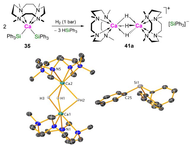
Scheme 10 Hydrogenolysis of compound 35 and molecular structure of dicalcium trihydride silylanide salt 41a .
