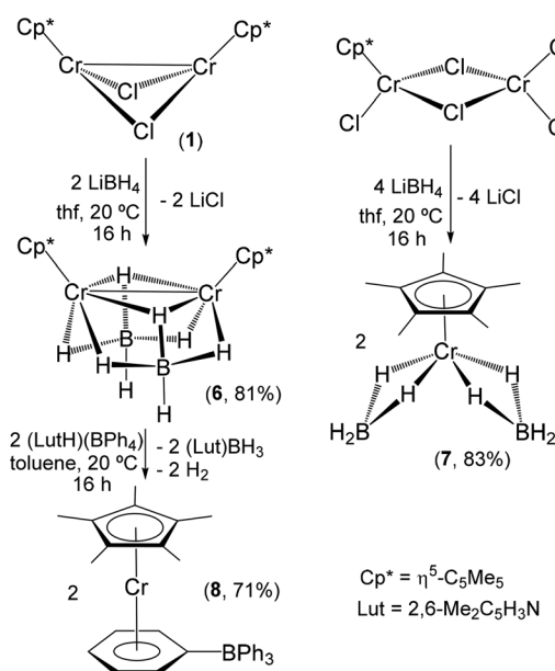
Scheme 3 Reactions of 1 and [\{\text{CrCp}^*\text{Cl}(\mu\text{-Cl})\}_2] with \text{LiBH}_4 .
