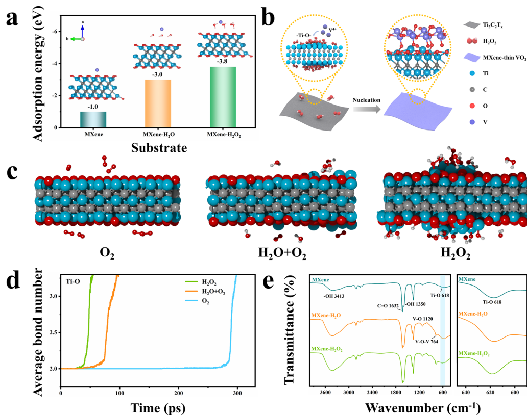
Fig. 2 Formation mechanism of the MXene- \text{VO}_{2-x} covalent heterostructure. (a) DFT calculation models for the adsorption of \text{V}^{4+} on the individual MXene, \text{H}_2\text{O} -anchored MXene (MXene- \text{H}_2\text{O} ), and \text{H}_2\text{O}_2 -anchored MXene (MXene- \text{H}_2\text{O}_2 ). (b) Schematic diagram of the predicted formation mechanism of the heterointerface. (c) MD simulated structure of MXene after oxidation in dry air ( \text{O}_2 ), wet air ( \text{H}_2\text{O} + \text{O}_2 ), and \text{H}_2\text{O}_2 environments after 25 ps at a temperature of 1000 K (Ti: blue, C: gray, and O: red). (d) Change in the average bond number of Ti-O under dry air, wet air, and \text{H}_2\text{O}_2 environments. (e) FTIR spectra of samples under dry air, wet air, and \text{H}_2\text{O}_2 environments.
