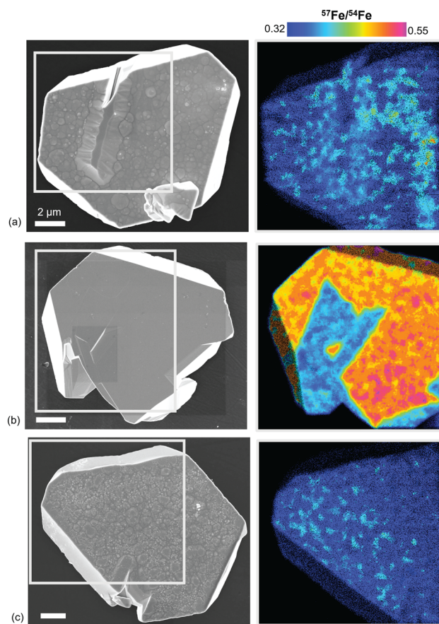
Fig. 5 Morphological characteristics shown by SEM and correlative NanoSIMS isotopic mapping on the (a) control ^{57}\text{Fe(II)} -oxalate-hematite, (b) ^{57}\text{Fe(II)} -hematite, (c) ^{57}\text{Fe(II)} -oxalate-hematite samples.
