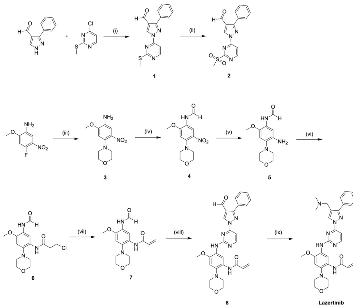
Scheme 1 A gram-scale preparation of lazertinib based on US20200207750A1 Yuhua Corp. patent. 42 Reagents and conditions are as follows: (i) K_2CO_3 , DMF, 50 °C, 2 h, 90%; (ii) 35% H_2O_2 (aq), (NH_4)_6Mo_7O_{24} \cdot 4H_2O , EtOH, rt, 2 h, 84%; (iii) morpholine, DIPEA, MeCN, rt, 4 h, 96%; (iv) HCO_2H , AcOH, THF, rt, 1 h, 91%; (v) NH_4HCO_2 , 10% Pd/C, EtOH, THF, 40 °C, 2 h, 68%; (vi) 3-chloropropionyl chloride, NaHCO_3 , MeCN, rt, 0.5 h; (vii) Et_3N , n -PrOH, rt, 3 h, 99% over last 2 steps; (viii) 2, t -BuONa, THF, rt, 1 h, 2 N NaOH (aq), rt, 15 h, 56%; (ix) Me_2NH \cdot HCl , DIPEA, DMA, rt, 1 h, STAB, rt, 1 h, 92%.
