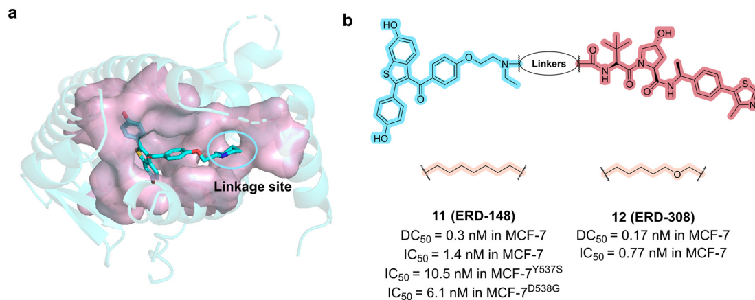
Fig. 6 a) X-ray structure of the crystal structure of raloxifene complexed with ER \alpha (PDB code: 7KBS). b) Chemical structures of compounds 11 (ERD-148) and 12 (ERD-308).
