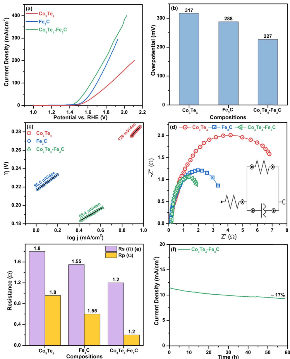
Fig. 4 OER electrocatalysis: (a) LSV curves, (b) bar chart of the overpotential at 10 \text{ mA cm}^{-2} current density, (c) Tafel plots, (d) EIS plots, (e) comparison of R_p and R_s , and (f) stability ( i - t ) curve of \text{Co}_3\text{Te}_4 , \text{Fe}_3\text{C} and \text{Co}_3\text{Te}_4\text{-Fe}_3\text{C} .
