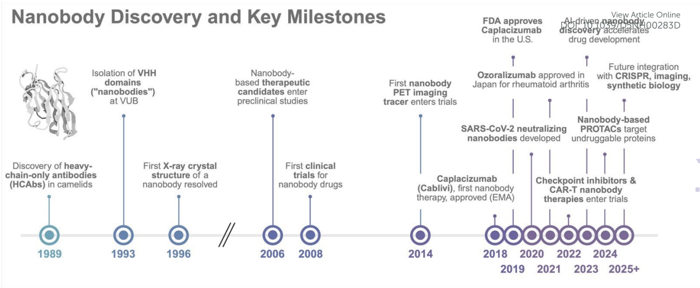
Fig. 1 A chronological overview highlighting major developments in nanobody research, from the initial isolation of camelid-derived nanobodies to the approval of nanobody-based therapeutics by the FDA. The figure includes a structural representation of a nanobody against Gelsolin (PDB ID: 2X1P). Created with Biorender.com.
