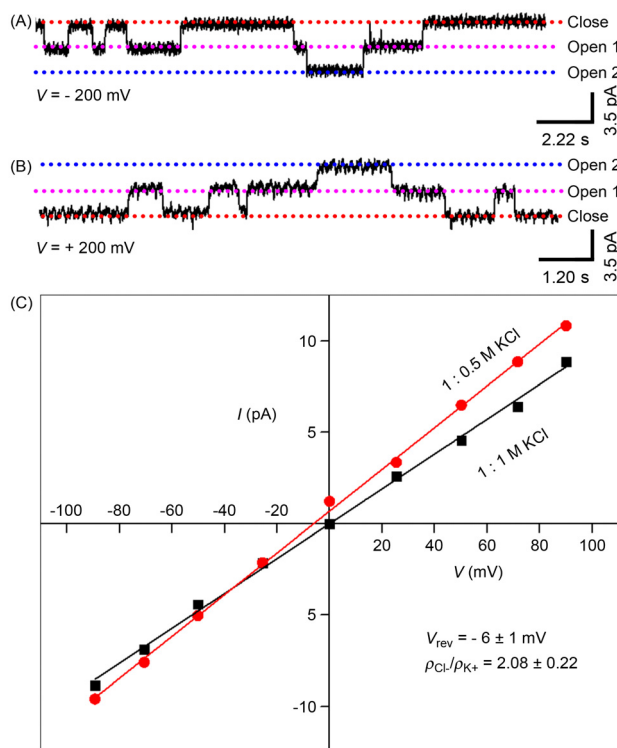
Fig. 3 Current traces recorded with 1d ( c = 2.0 \mu\text{M} ) at -200 mV (A) and +200 mV (B) in a symmetrical KCl solution. Current-voltage relationship of 1d in both symmetrical and asymmetrical KCl concentrations (C).
