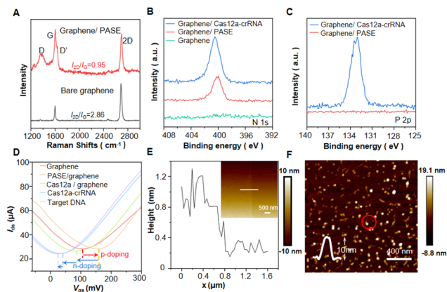
Fig. 2 Device characterization. (A) Raman spectra of bare graphene and PASE/graphene. (B) XPS N 1s peak of bare graphene and that after modified with PASE and Cas12a-crRNA. (C) XPS P 2p peak of graphene modified with PASE and Cas12a-crRNA. (D) Transfer curves of bare graphene that is modified with PASE, Cas12a, and Cas12a-crRNA RPN and that binds with target DNA. (E and F) AFM images (tapping mode in air) of bare graphene and graphene modified with Cas12a. The scale bars are 500 nm in (E) and 400 nm in (F).
