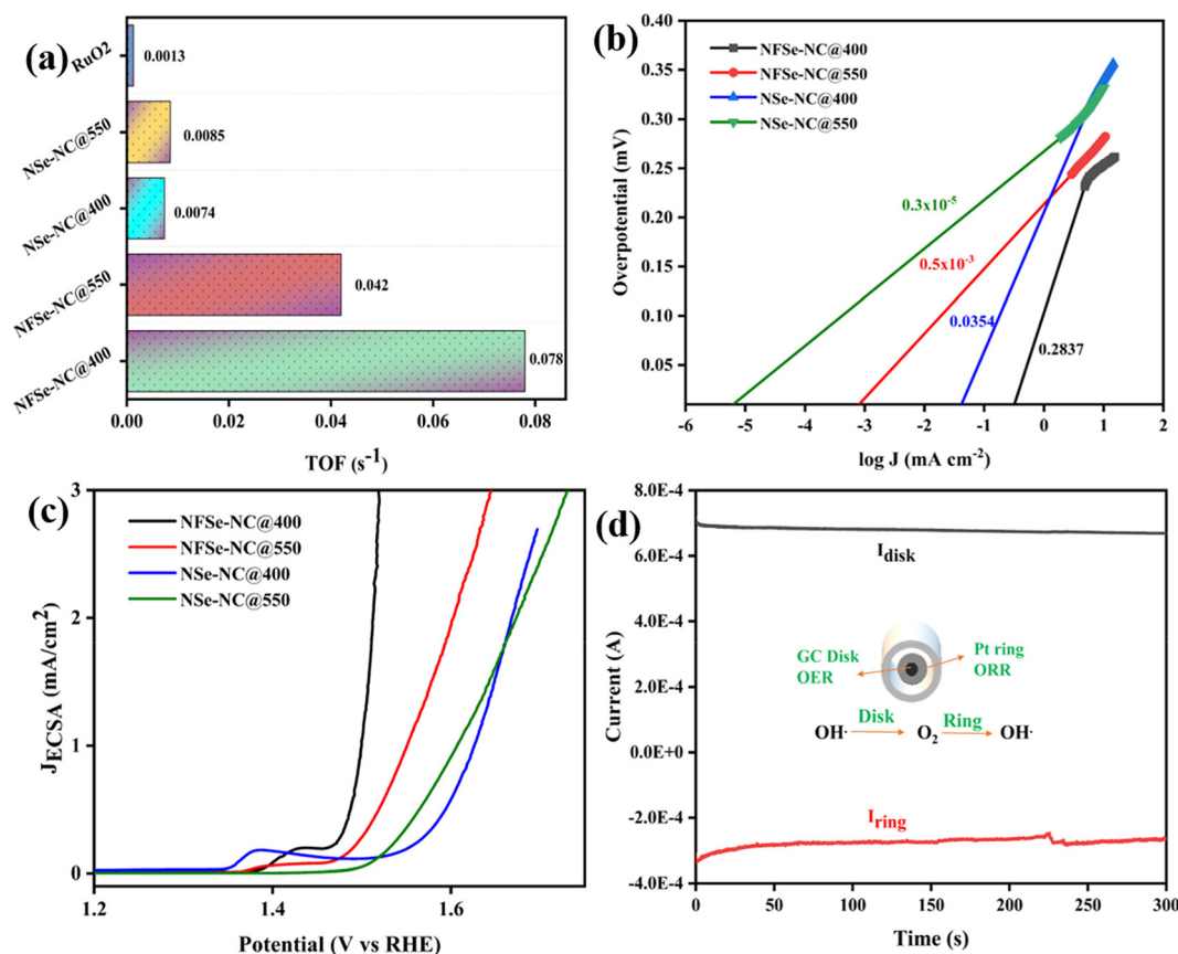
Fig. 7 (a) TOF values at 1.49 V, (b) exchange current density, (c) ECSA derived LSV of different electrocatalysts, and (d) faradaic efficiency measurement using RRDE for \text{NFSe-NC@400} .
