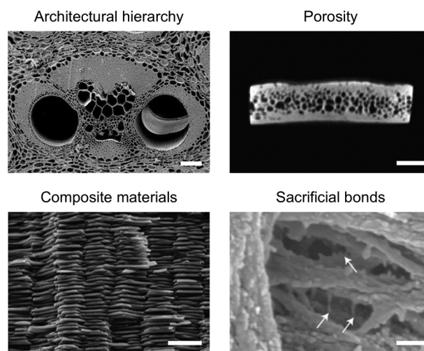
Fig. 1 Biological strategies to achieve impact resistance in natural materials. Top left to bottom right: architectural hierarchy in bamboo's culm wall (SEM, scale bar: 100 µm; adapted from ref. 11, copyright 2010 Budapest University of Technology and Economics); porosity in a turtle's shell (X-ray CT, scale bar: 2 mm; reprinted from ref. 12 with permission from Elsevier, copyright 2009); composite materials such as nacre in seawater snails (SEM, scale bar: 10 µm; reprinted from ref. 13 with permission from Elsevier, copyright 2008), and collagen-based sacrificial bonds [white arrows] within fractured bone (AFM, scale bar: 200 nm; adapted from ref. 14 with permission from Springer Nature, copyright 2005).
