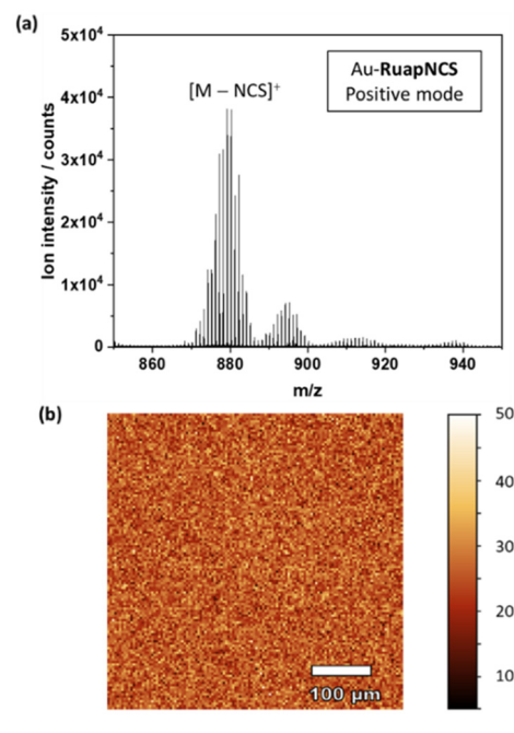
Fig. 3 (a) ToF-SIMS spectrum of ions derived from \text{Au-RuapNCS} in the positive mode. (b) 2D ToF-SIMS mapping for [\text{M} - \text{SCN}]^+ ions.
