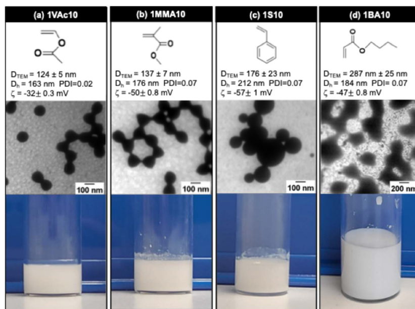
Fig. 8 TEM images and photographs of surfactant-free latex dispersions prepared via photo-SFEP under 405 nm irradiation at R = 1\text{‰} and \text{SC} = 10\% w/w of various monomers: (a) vinyl acetate (VAc), (b) methyl methacrylate (MMA), (c) and styrene (S), and (d) n -butyl acrylate (BA).
