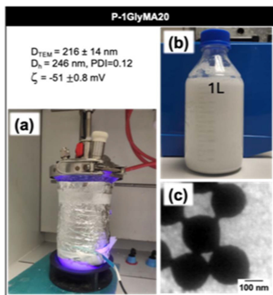
Fig. 7 Scale-up of surfactant-free latex synthesis via photo-SFEP of GlyMA under 405 nm irradiation. (a) Reaction setup for the scale-up to 1 liter, using R = 1\text{‰} and \text{SC} = 20\% w/w. (b) The resulting stable latex dispersion produced in a 1 L batch. (c) TEM image of nanoparticles in the latex.
