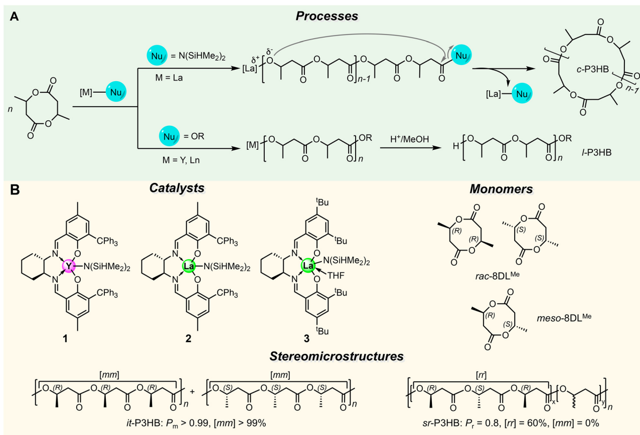
Fig. 1 (A) Sketched synthetic pathways from dimethyl diolide (8DLM Me ) to linear (l) and cyclic (c) P3HB. (B) Selected catalysts, monomers, and stereomicrostructures of P3HB discussed herein. All it-P3HB discussed is stereo-perfect, with [mm] > 99\% .
