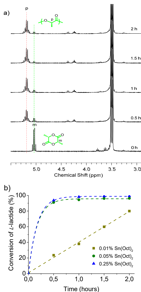
Figure 1 (a) ^1\text{H} -NMR ( \text{CDCl}_3 ) spectra of the \text{PLLA}_{21}\text{-}b\text{-PO3G}_{41}\text{-}b\text{-PLA}_{21} copolymer at different reaction times using 0.05% \text{Sn}(\text{Oct})_2 catalyst and, (b) conversion of L -lactide in the ROP initiated by the \text{PO3G}_{41} macroinitiator at different catalyst concentrations.
