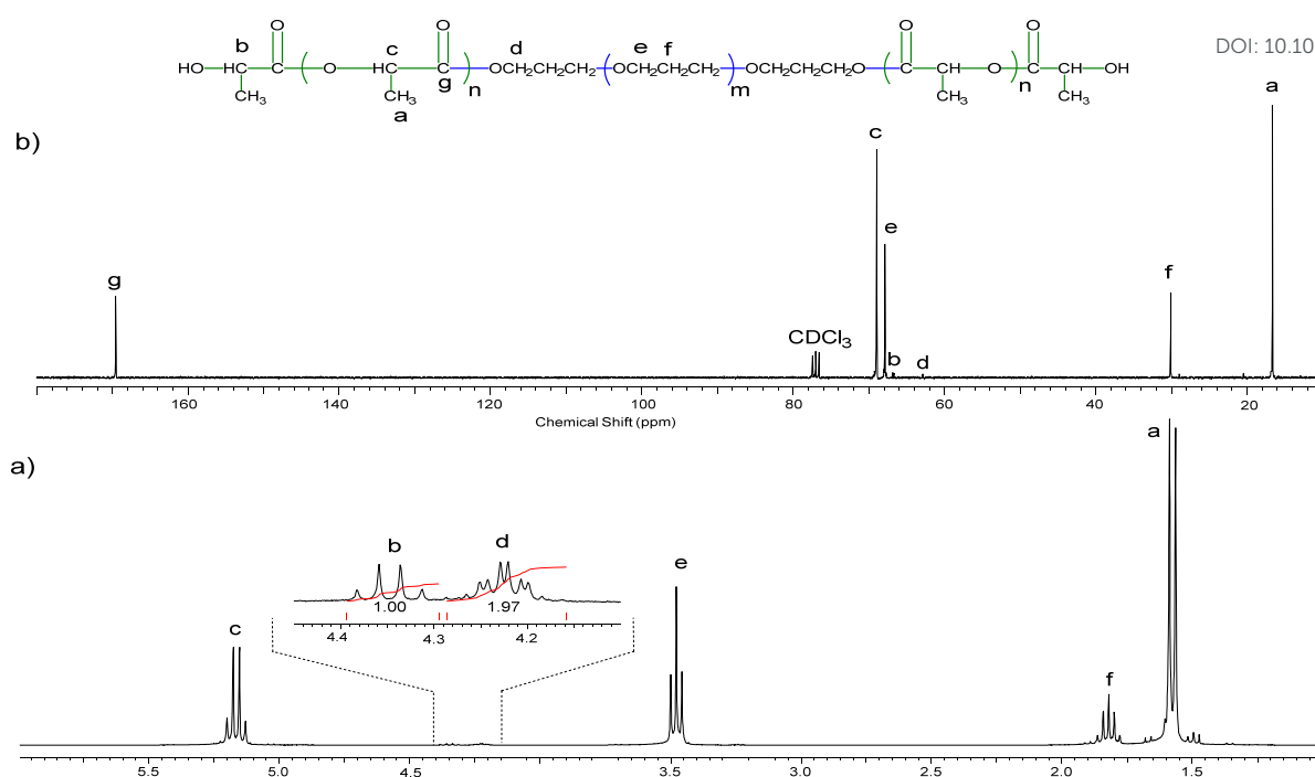
Figure 3 (a) ^1\text{H} - and (b) ^{13}\text{C} -NMR spectrum in \text{CDCl}_3 of \text{PLLA}_{82}\text{-}b\text{-PO3G}_{41}\text{-PLLA}_{82} copolymer
