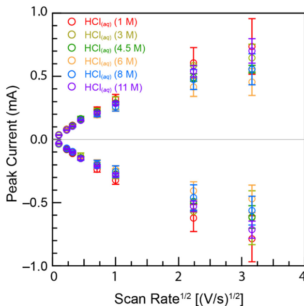
Fig. 6 Peak current ( i p ) from cyclic voltametric measurements made on plutonium (16.7 mM) in HCl (aq) (1–11 M) solutions plotted as a function of scan rate (0.01–10 V s -1 ). Error bars are the standard deviation from three replicates.
