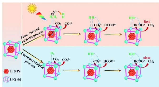
Figure 28. Proposed mechanism using Ir@UiO-66 for the thermal and photo-thermal catalytic Sabatier reaction process. Reprinted with permission from 101 . Copyright 2025 Royal Society of Chemistry.
