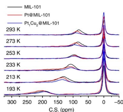
Figure 25. Temperature-dependent hyperpolarised 129 Xe NMR spectra for MIL-101, Pt@MIL-101, and PtCu@MIL-101 at temperatures ranging from 193–293 K. Reprinted with permission from 91 . Copyright 2025 Springer Nature.
