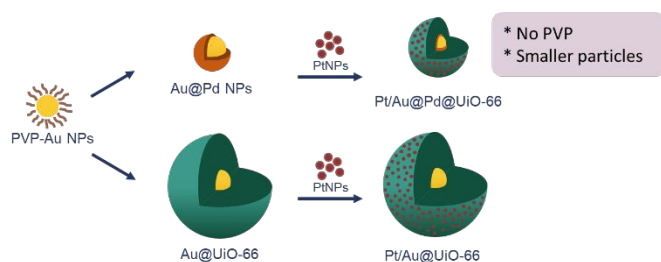
Figure 8. Schematic representation of the two synthetic routes taken to centrally encapsulate AuNPs or Au@PdNPs with uniform dispersion of PtNPs, resulting in Pt/Au@Pd@UiO-66 and Pt/Au@UiO-66 for gas-phase CO 2 hydrogenation through RWGS. Adapted with permission from 44 . Copyright 2025 John Wiley and Sons.
