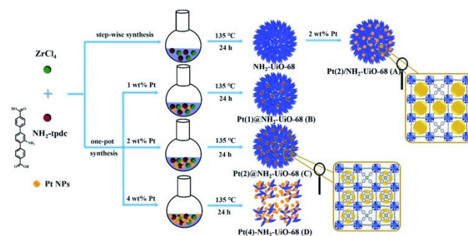
Figure 12. Schematic diagram of the two synthesis routes described by Guo et al.: step-wise synthesis of \text{Pt}/\text{NH}_2\text{-UiO-68} and one-pot synthesis of \text{Pt}@\text{NH}_2\text{-UiO-68} . Reprinted with permission from 54 . Copyright 2025 Royal Society of Chemistry
