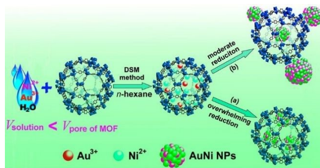
Figure 3. Schematic diagram of the double solvent method (DSM) for the immobilisation of AuNi nanoparticles on a Cr-MIL-101 matrix. (a) Overwhelming reduction is achieved using an excess of reducing agent compared to the MOF pore volume to achieve full reduction and small nanoparticles. (b) Moderate reduction is the result of a lower reductant concentration, resulting in agglomeration and larger nanoparticles due to the ability of the nanoparticles to dissolve and leach to the surface. Reprinted with permission from 32 . Copyright 2025 American Chemical Society.
