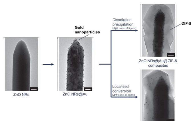
Figure 10. Schematic representation for the spatial regulation using the sacrificial-template synthetic method for the surface modification. TEM images of ZnONRs, ZnONRs@AuNPs, and ZnONRs@AuNPs@ZIF-8 composites with AuNPs at different locations as the result of dissolution precipitation or localised conversion. The Scale bar is 100 nm. Adapted with permission from 51 . Copyright 2025 Springer Nature.
