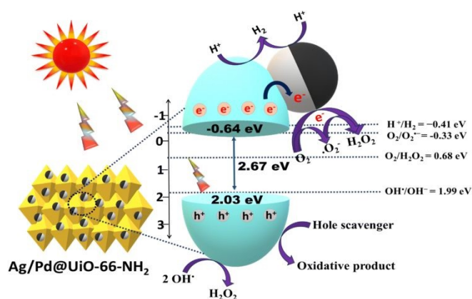
Figure 28. Schematic representation of the mechanistic pathway for H 2 O 2 and H 2 evolution using Ag/Pd@UiO-66-NH 2 as a photocatalyst, including the ability of Ag/PdNPs to act as electron traps to limit electron pair recombination. Reprinted with permission from 21 . Copyright 2025 Royal Society of Chemistry.
