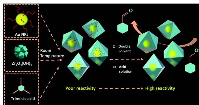
Figure 7. Schematic diagram for the assembly of AuNPs@MOF-808 composites using PVP stabilised AuNPs, Zr 6 O 4 (OH) 4 and trimesic acid by DSM at room temperature. The PVP removal from the AuNPs by acid treatment resulted in enhanced catalytic activity for the reduction of benzyl alcohol to benzaldehyde. Reprinted with permission from 43 . Copyright 2025 Royal Society of Chemistry.
