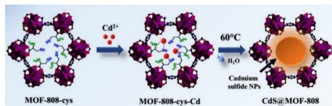
Figure 16. Synthesis scheme of CdS@MOF-808 composites produced by post-synthetic ligand exchange (PSLE) of MOF-808 with L-cysteine (L-cys), followed by the growth of CdSNPs after temperature treatment. Reprinted with permission from 7 . Copyright 2025 American Chemical Society.
