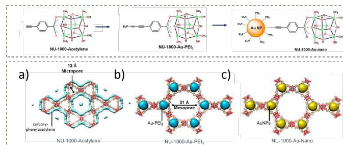
Figure 23. Different envelope density (DED) maps showing the location of a) carboxy-phenylacetylene in NU-1000-Acetylene and b) Au-PET 3 in NU-1000-Au-PET 3 . Adapted with permission from 12 . Copyright 2025 American Chemical Society.
