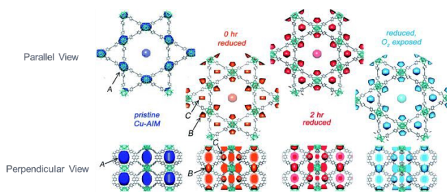
Figure 24. DED maps showing parallel (top) and perpendicular (bottom) views of c-axis for Cu-AIM in the pristine state (dark blue), at the beginning (red) and end of reduction at 200 °C (pink) and following re-oxidation (light blue). Adapted with permission from 11 . Copyright 2025 Royal Society of Chemistry.
