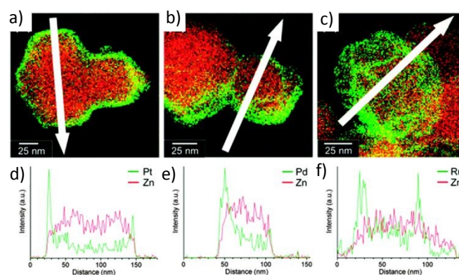
Figure 20. STEM-EDS maps of (a) Pt/ZIF-8, (b) Pd/ZIF-8, and (c) Ru/ZIF-8. Line profiles of (d) Pt/ZIF-8, (e) Pd/ZIF-8, and (f) Ru/ZIF-8 along white arrows (green: Pt-M, Pd-L, or Ru-L; red: Zn-K). Adapted with permission from 63 . Copyright 2025 Royal Society of Chemistry.
