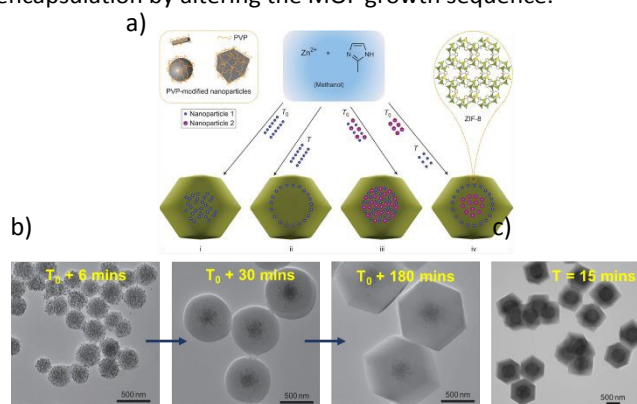
Figure 13. a) A diagram showing how the addition sequence of the PVP-modified nanoparticles during MOF synthesis played a role in the spatial distribution of the incorporated PVP-modified nanoparticles within the ZIF-8 crystals at T_0 or T during the MOF synthesis, b) TEM images of the intermediate products of Au nanoparticle/ZIF-8 hybrid crystals collected at different reaction times: 6 minutes, 30 minutes, and 180 minutes after nanoparticle addition, c) TEM image of hybrid crystals obtained when Au nanoparticles AuNPs were added 15 minutes after the initiation of the reaction. Adapted with permission from 57 . Copyright 2025 Springer Nature.
