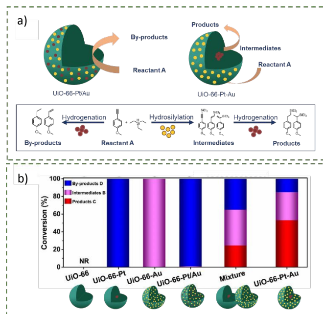
Figure 27. a) Scheme of hydrosilylation–hydrogenation tandem reaction catalysed by UiO-66-Pt-Au, or the formation of by-products due to the favourable hydrogenation reaction with UiO-66-Pt/Au. b) Catalytic performance of various precursors and catalysts in the study based on conversion to by-products, intermediates, or products. Adapted with permission from 3 . Copyright 2025 Springer Nature.
