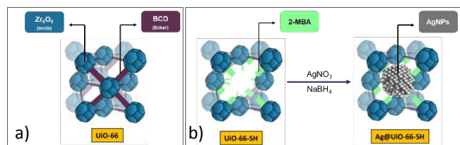
Figure 17. a) A diagram of UiO-66 and b) schematic representation for the synthesis of Ag@UiO-66-SH composite using defective UiO-66-SH with AgNO 3 as the silver source, then reduced with NaBH 4 . Adapted with permission from 73 . Copyright 2025 American Chemical Society.
