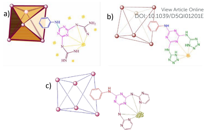
Figure 18. Simplified structures of a) UiO-66-NH 2 @cyanuric chloride@guanidine/PdNPs, 77 b) UiO-66-NH 2 @cyanuric chloride@5-amino tetrazole/AuNPs, 78 and c) UiO-66-NH 2 @cyanuric chloride@2-aminopyrimidine/PdNPs. 79 Adapted with permission from 77,79 . Copyright 2025 American Chemical Society. Adapted with permission from 78 . Copyright 2025 Springer Nature.
