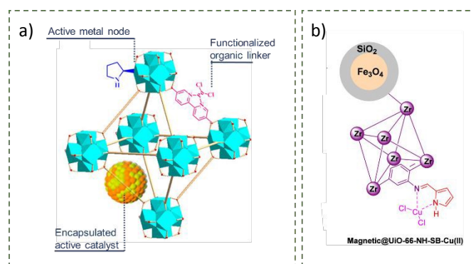
Figure 29. Schematic representation of multifunctional MOF composites, a) novel trifunctional chiral heterogeneous MOF catalyst. Adapted with permission from 114 . Copyright 2025 American Chemical Society, b) magnetic@UiO-66-NH-SB-Cu(II). Reprinted with permission from 115 . Copyright 2025 American Chemical Society.
