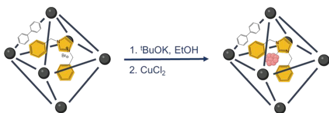
Figure 19. Synthesis reaction scheme to produce 2Bn-Cu@UiO-67 from UiO-67-NHC by addition of base and copper salt. Adapted) with permission from 88 . Copyright 2025 John Wiley and Sons.
