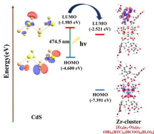
Figure 26. HOMO–LUMO energy positioning (eV) of the CdS-photosensitizer and Zr 4+ cluster as catalysts for HER. The photoinduced electron transfer (PET) (H atoms have been omitted for clarity) is also illustrated. Reprinted with permission from 7 . Copyright 2025 American Chemical Society.
