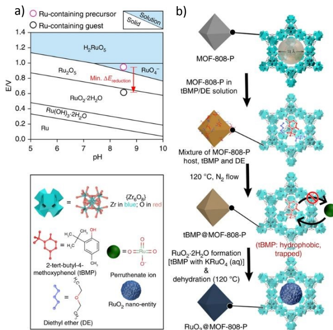
Figure 14. a) The Pourbaix diagram for the Ru-H 2 O system, b) Schematic diagram of the Pourbaix-enabled guest synthesis (PEGS) strategy for \text{RuO}_2 @MOF-808-P. Reprinted with permission from 58 . Copyright 2025 Springer Nature.
