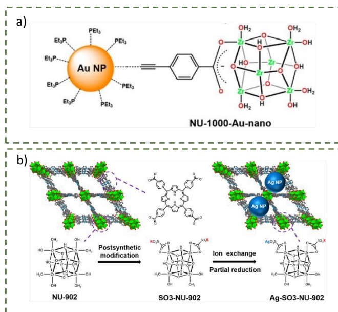
Figure 2. a) Structure of NU-1000-Au-nano (NU-1000 = [\text{Zr}_6(\mu_3\text{-O})_4(\mu_3\text{-OH})_4(\text{OH})_4(\text{H}_2\text{O})_4(\text{TBAPy})_2]_{\infty} ) where the AuNP is bound to the MOF via the acetylene group of the carboxy-phenylacetylene linkers. Reprinted with permission from 12 . Copyright 2025 American Chemical Society. b) Schematic representation of the synthesis route of Ag-SO3-NU-902. Reprinted (adapted) with permission from 25 . Copyright 2025 American Chemical Society.
