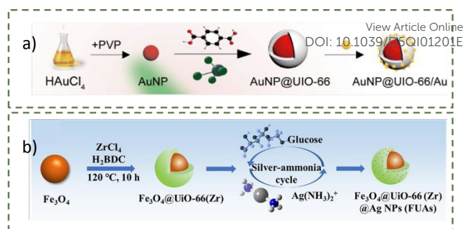
Figure 9. Schematic diagram of the fabrication of a) AuNP@UiO-66/Au nanoparticles 49 and b) Fe 3 O 4 @UiO-66(Zr)@AgNPs 50 . Reprinted with permission from 49 . Copyright 2025 Royal Society of Chemistry. Reprinted with permission from 50 . Copyright 2025, with permission from Elsevier.
