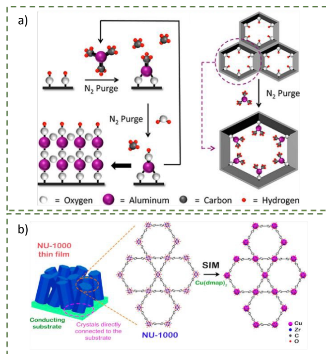
Figure 5. a) Schematic representation of the vapour-phase atomic layer deposition (ALD) in MOFs (AIM). Reprinted with permission from 37 . Copyright 2025 American Chemical Society. b) Schematic representation of the solvothermal deposition in MOFs (SIM). Reprinted with permission from 38 . Copyright 2025 American Chemical Society.
