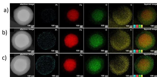
Figure 21. Electron image, elemental mapping images, and EDX layered images of (a) Fe 3 O 4 @MIL-100(Fe)-Pt(10), (b) Fe 3 O 4 @MIL-100(Fe)-Pt(20), and (c) Fe 3 O 4 @MIL-100(Fe)-Pt(30). Adapted with permission from 52 . Copyright 2025 American Chemical Society.
