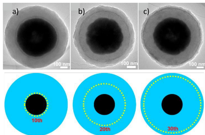
Figure 11. TEM images of a) \text{Fe}_3\text{O}_4@\text{MIL-100}(\text{Fe})\text{-Pt}(10) , b) \text{Fe}_3\text{O}_4@\text{MIL-100}(\text{Fe})\text{-Pt}(20) , and c) \text{Fe}_3\text{O}_4@\text{MIL-100}(\text{Fe})\text{-Pt}(30) with schematic representation below each image. Adapted with permission from 52 . Copyright 2025 American Chemical Society.
