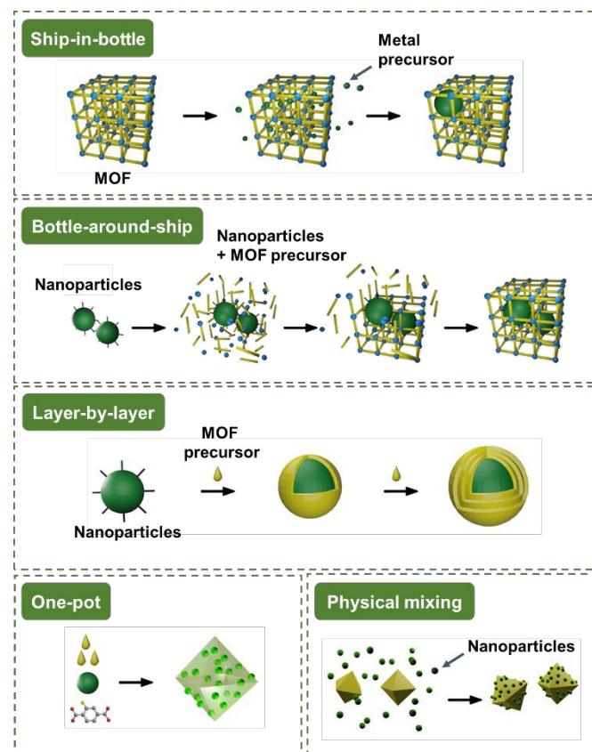
Figure 1. Schematic diagram of the different synthetic methods to form a nanoparticle-MOF composite: “ship-in-bottle” strategy, “bottle-around-ship” strategy, “layer-by-layer” strategy, “one-pot” strategy, and physical mixing strategy. Adapted from 19 , Copyright 2025, with permission from Elsevier.
