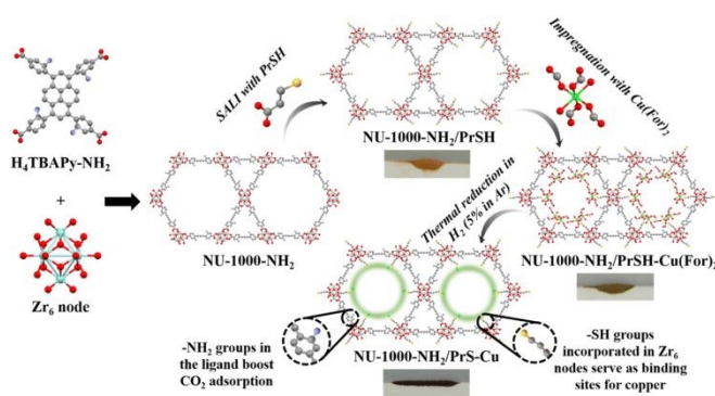
Figure 15. Schematic representation of the synthesis procedure to produce NU-1000-NH 2 /PrSH-Cu, highlighting the reasoning behind the installed functionalities and the difference in colour of the powders during the synthesis steps. Reprinted with permission from 24 . Copyright 2025 Royal Society of Chemistry
