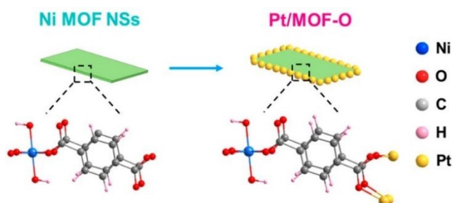
Figure 4. Schematic representation of site-specific growth of PtNPs on the edge of two-dimensional (2D) heterojunction Ni-MOFs using ethylene glycol (EG) or diethyl glycol (DEG) as reducing agent. Reprinted with permission from 34 . Copyright 2025 American Chemical Society.
