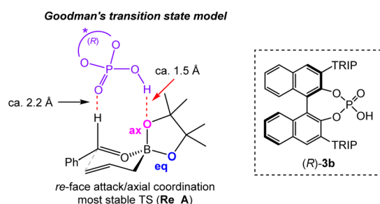
Fig. 2 Goodman's transition state model.
