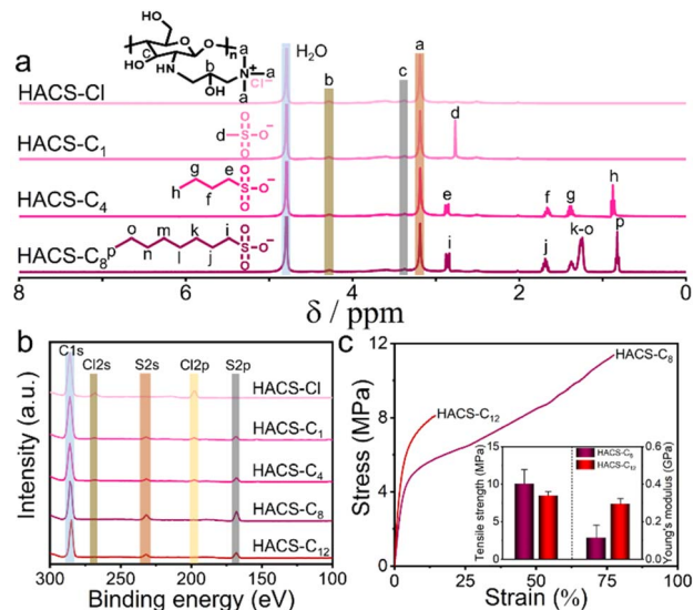
Fig. 1 Characterization of cationic polyelectrolytes HACSCl with different monovalent counterions. (a) ^1\text{H} NMR spectra and (b) XPS analyses of HACSCl and HACSC x materials. (c) Representative stress-strain curves for HACSC 8 and HACSC 12 with the inset showing the tensile strengths and Young's moduli.
