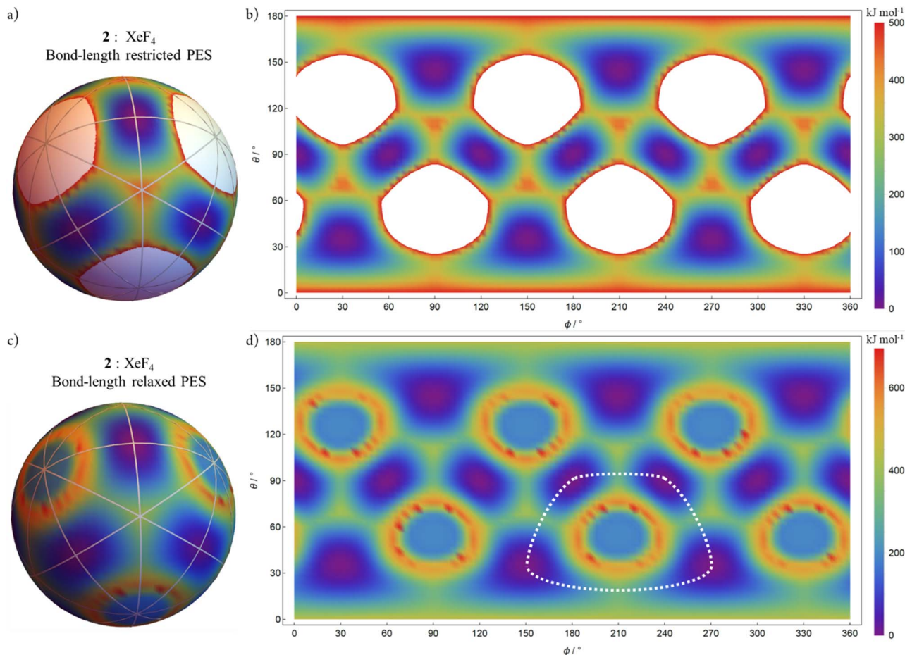
Fig. 8 AB_4 T-4 E-mode qualitative potential energy surfaces (PESs) for \text{XeF}_4 . (a) Bond-length restricted PES (Xe–F fixed at the local-minimum geometry length) corresponding to the spherical configuration space with an energy cutoff of 500 \text{ kJ mol}^{-1} . (b) An “equirectangular projection” of the spherical PES from (a). (c) Bond-length relaxed PES for \text{XeF}_4 corresponding to the spherical configuration space. (d) An “equirectangular projection” of the spherical PES from (c). There are 12 local minimum wells (purple) corresponding to square planar SP-4 geometries. The white dashed lines indicate polytopal rearrangement trajectories through the configuration space that avoid the high energy regions centred on the symmetric linear SL-4 species. For (a) and (c), the 9 great circles of the disdyakis dodecahedron are shown.
