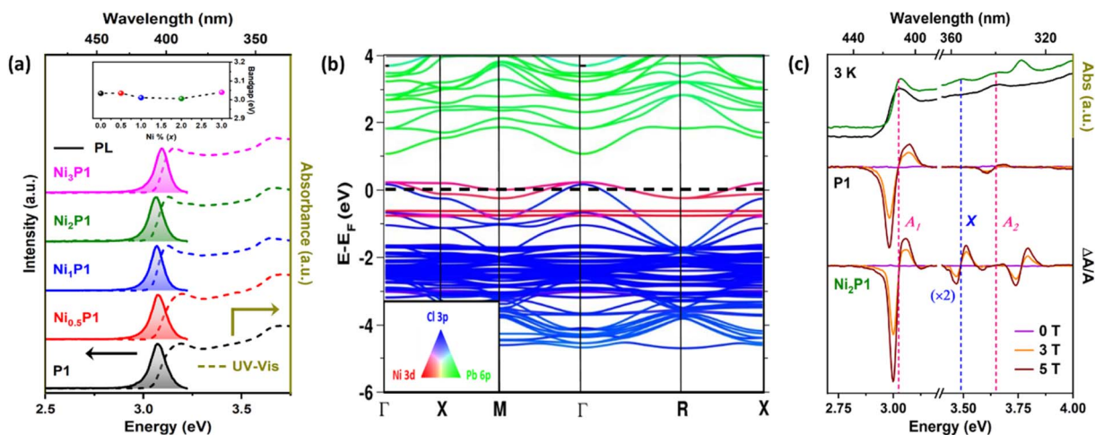
Fig. 2 Optical and electronic properties: (a) room temperature absorption and emission spectra of undoped (P1) and various Ni-doped CsPbCl 3 (Ni x P1; x = 0, 0.5, 1, 2, 3 ) NCs with the inset of bandgap variation with different Ni-percentage (dashed line guides to the eye) showing a bowing effect. (b) Orbital projected band structure of Ni-doped CsPbCl 3 with considering spin-orbit coupling (SOC). Red, green, and blue colors represent Ni 3d, Pb 6p, and Cl 3p atomic orbitals respectively, while intermediate colors indicate the extent of mixing or hybridization of these orbital contributions. Band structure confirms significant hybridization of Ni 3d and Cl 3p orbitals near the VBM at \Gamma point. (c) MCD spectra of P1 and Ni 2 P1 with their absorption at temperature 3 K with varying magnetic field (0, 3, and 5 T). The presence of extra differential peak (X) confirms the Ni 2+ -induced exchange interaction.
