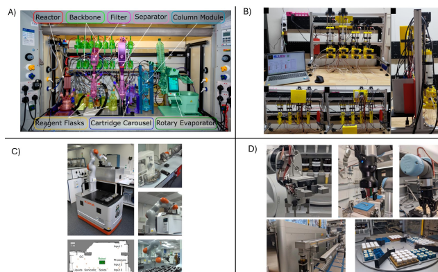
Fig. 2 Examples of robotics and automation developed and adopted in chemistry laboratories. A) Modular, universal ChemPU platform. from 40 with permission. B) FLUID Reprinted with permission from 33 . Copyright 2025 American Chemical Society. C) a Kuka mobile robot platform and its operating environment. Reprinted with permission from 35 . D) UR5e robotic arms used for sample preparation, retrieval, and characterization. Reprinted with permission from 36 .
