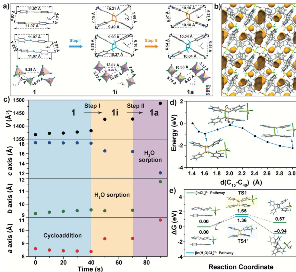
Fig. 2 (a) Geometrical variation of \text{LH}^+ dimers and the [\text{InCl}_5]^{2-} polyhedron in 1 , 1i , and 1a . (b) Schematic illustration of the free volume in 1i (probe radius: 1.0 \text{\AA} ; approx. grid spacing: 0.2 \text{\AA} ). (c) Lattice parameters of 1 at different irradiation times (light source: 450 nm, 260 \text{mW cm}^{-2} ). (d) Energy profile of the [2 + 2] cycloaddition reaction with constrained C-C bond length. The \text{C}_{15}-\text{C}_{40} bond length was fixed during the optimization process to examine the impact of this constraint on the reaction pathway. (e) Computational study of \text{LH}^+ dimers, the [\text{InCl}_5]^{2-} polyhedron, \text{LH}^+ photodimers, and the [\text{In}(\text{H}_2\text{O})\text{Cl}_5]^{2-} octahedron involved in [2 + 2] cycloaddition reactions.
