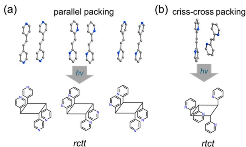
Figure 3. Different conformations of cyclobutane photoproducts.
