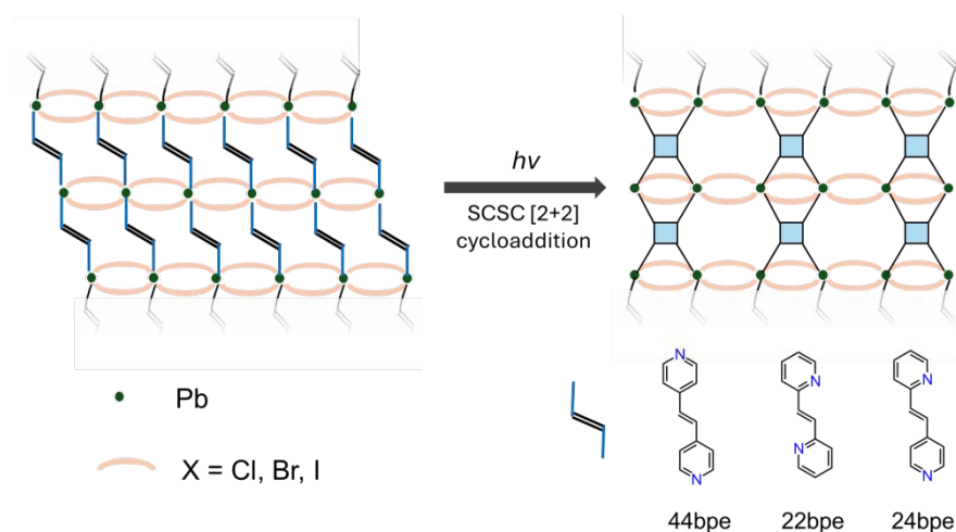
Scheme 1. Schematic illustration for the design of lead halide coordination polymers and their solid-state [2+2] photocycloaddition process.
