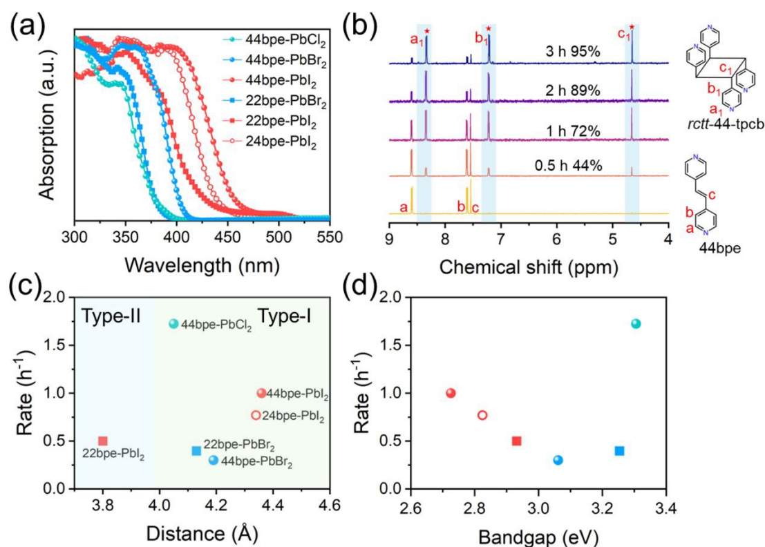
Figure 2. (a) Absorption spectrum of the bpe-PbX 2 CPs. (b) 1 H NMR spectra of the 44bpe-PbCl 2 under different irradiation times. (c) Photocycloaddition rates of the bpe-PbX 2 CPs with different double bond distances. (d) The relationship between the photocycloaddition rates and bandgap.
