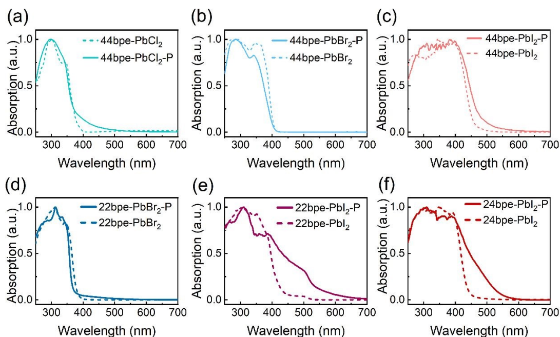
Figure 5. Absorption spectrum changes in bpe-PbX 2 CPs after photocycloaddition. (a), 44bpe-PbCl 2 . (b), 44bpe-PbBr 2 . (c), 44bpe-PbI 2 . (d), 22bpe-PbBr 2 . (e), 22bpe-PbI 2 . (f), 24bpe-PbI 2 .
