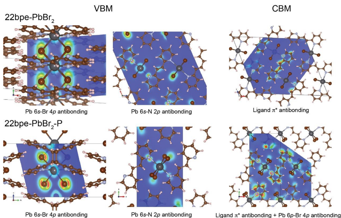
Figure 7. Band decomposed partial charge densities of 22bpe-PbBr 2 (top panel) and 22bpe-PbBr 2 -P (bottom panel) at VBM (left and middle panels) and CBM (right panel), respectively.
