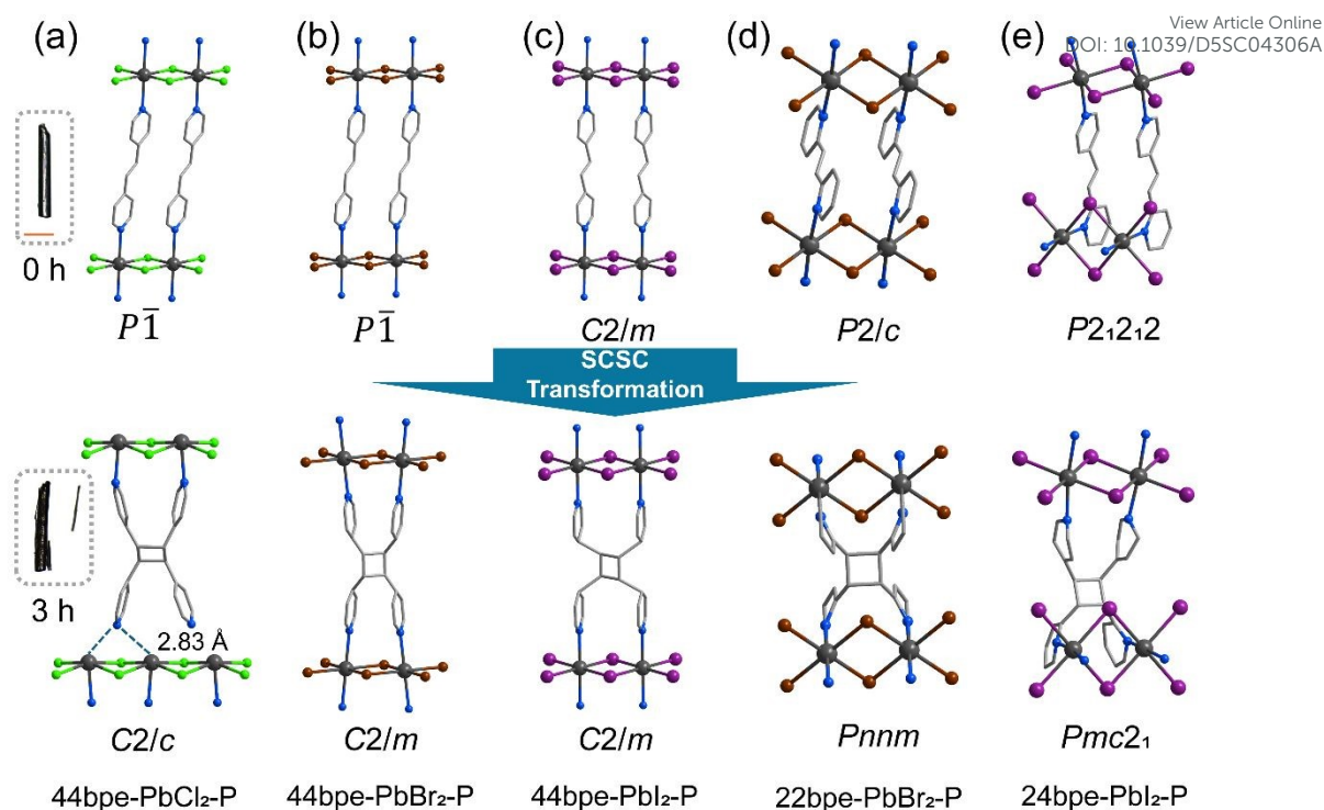
Figure 4. [2+2] Photocycloaddition induced SCSC transformation in bpe-PbX 2 CPs. (a), 44bpe-PbCl 2 -P, inserted photo corresponds to the single crystal after illumination, scale bar is 100 μm. (b), 44bpe-PbBr 2 -P. (c), 44bpe-PbI 2 -P. (d), 22bpe-PbBr 2 -P. (e), 24bpe-PbI 2 -P.
