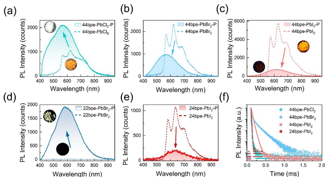
Figure 6. Photocycloaddition-induced PL spectrum changes in 44bpe-PbCl 2 (a), 44bpe-PbBr 2 (b), 44bpe-PbI 2 (c), 22bpe-PbBr 2 (d), 24bpe-PbI 2 (e). (f), PL lifetime of the bpe-PbX 2 CPs.
