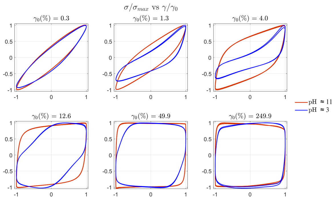
Fig. 11 Normalised elastic Lissajous–Bowditch (LB) plots ( \sigma/\sigma_0 vs. \gamma/\gamma_0 ) for STO formulations: STO47 L5(2) at pH ≈ 11 and ≈3 before and after aggregation respectively. LB curves for the aggregated sample at pH ≈ 3 are asymmetric at intermediate values of strain amplitude that correspond to the increase of even harmonics, I_{2/1} in Fig. 10(b), between \gamma_0 \approx 0.015 and 10%.
