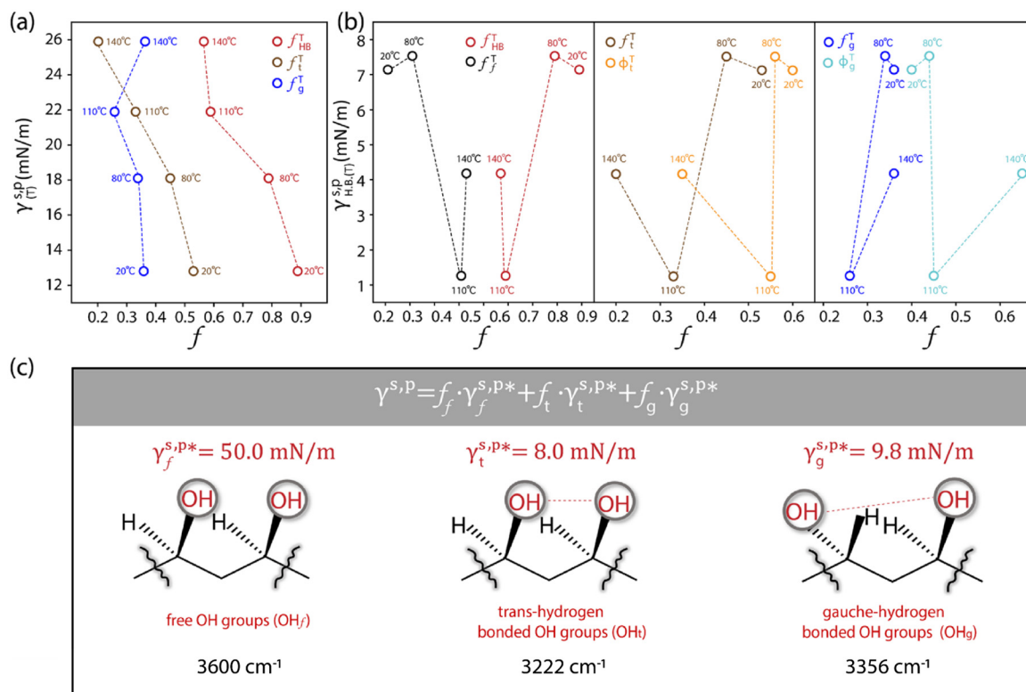
Fig. 3 (a) Plots of the \gamma_{(T)}^{S,P} values of the as-prepared L_PVA 2 thin films versus their f_{HB}^T , f_t^T , and f_g^T values. (b) Plots of the \gamma_{H,B(T)}^{S,P} values of the as-prepared L_PVA 2 thin films versus their f_{HB}^T ( f_t^T ) (left panel), f_t^T ( \phi_t^T ) (middle panel), and f_g^T ( \phi_g^T ) values (right panel). (c) Schematic summarizing the molecular configurations of the surface OH f , OH g , and OH t groups, with the corresponding \gamma_f^{S,P*} , \gamma_g^{S,P*} , and \gamma_t^{S,P*} values marked.
