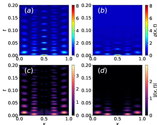
Fig. 6 Dynamics. The color map indicates the time evolution of the density field \rho(x, t) from an initial Gaussian distribution centered in L/2 ( L = 1 ). Different panels display different values of the tumbling rate \alpha = 0.1, 2 (panels (a) and (b), respectively). Panels (c) and (d) show the intensity of the corresponding current fields |J(x, t)| . At small \alpha value, the system clearly support traveling damped waves that become more and more damped as \alpha increases.
